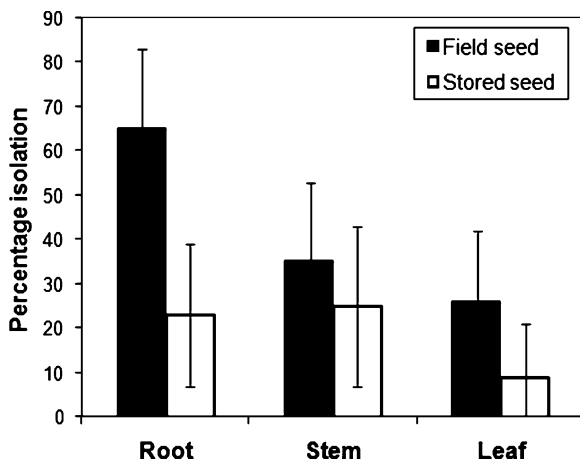
Fig. 1 Incidence of B. cinerea in tissues sampled from lettuce plants cv. Tom Thumb grown in a filtered, spore-free, air-flow, in relation to seed-source. Before planting, field seed had a high incidence of B. cinerea and stored seed, a low incidence. Error bars are 2 se derived from the generalised linear model used to analyse the data
